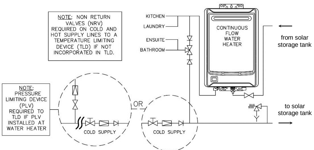
In-series Gas Booster as part of a Closed Circuit Solar Water Heater Installation Two Temperature Zones Using a Temperature Limiting Device
